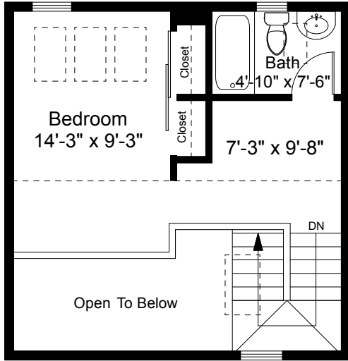
Third Floor Plan Ceiling Height = 12'-2"
