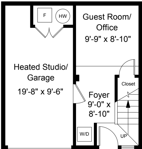
First Floor Plan Ceiling Height = 7'-1"
